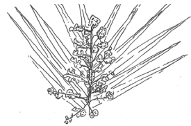
inflorescence
